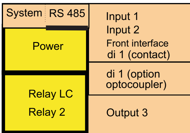
Fig.1: galvanic isolation
