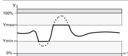
Fig.: 33 Fixed positioning limits
