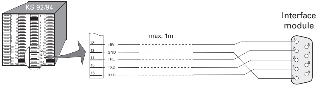
Fig.: 2 RS422-interface connection
