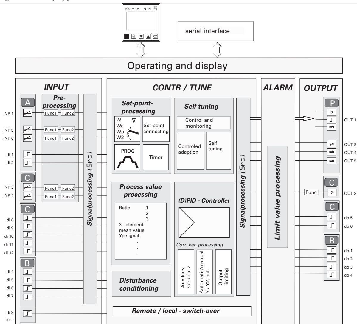
Fig.: 11 Survey of functions
