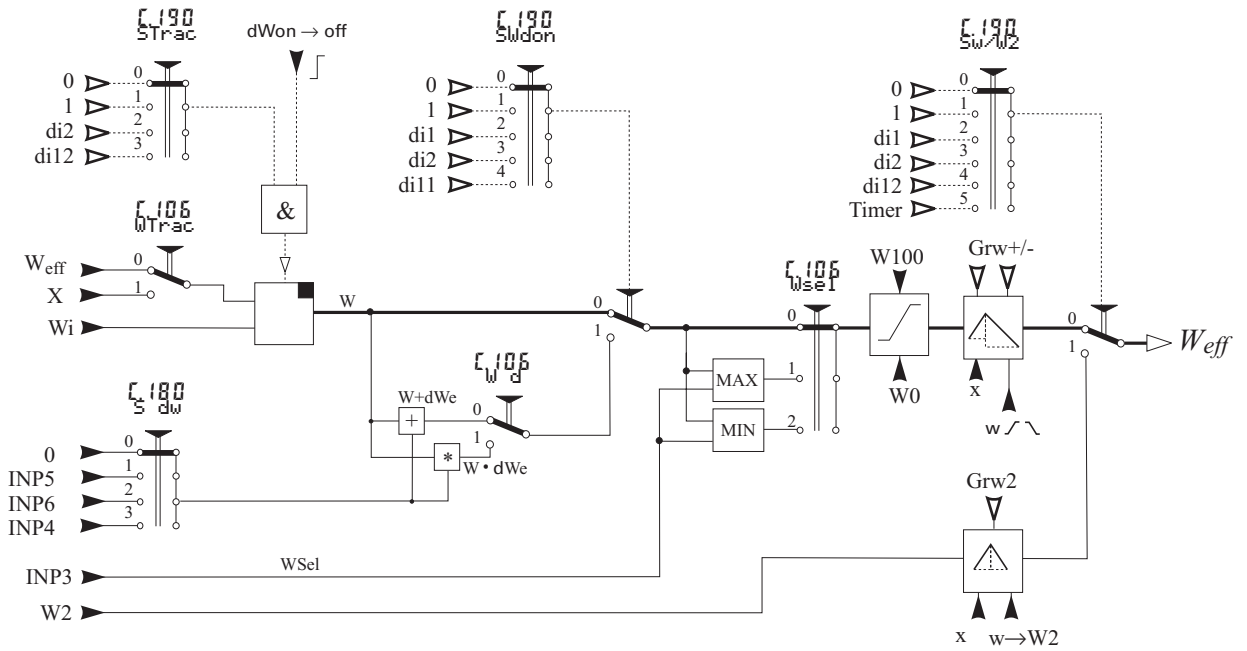
Fig.: 15 Set-point control with external offset \epsilon_{.100} ; WFunc = 3
