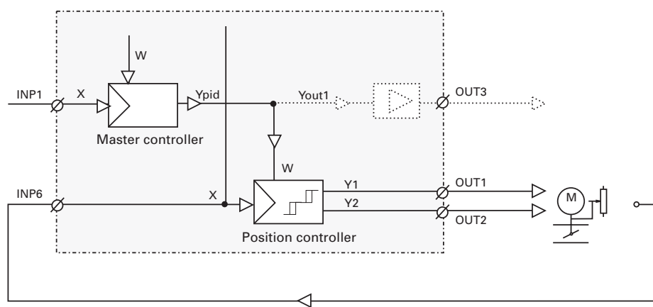
Fig.: 56 Continuous controller with position controller
