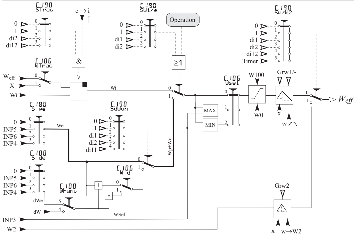
Fig.: 16 Setpoint / cascade control with offset \epsilon_{.100} ; WFunc = 4/5
